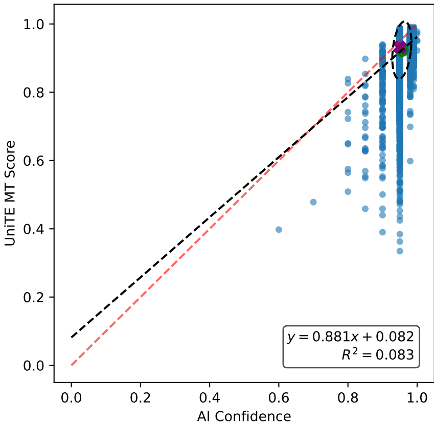
Calibration of Qwen3-14B basic on Chinese with monolithic prompt
