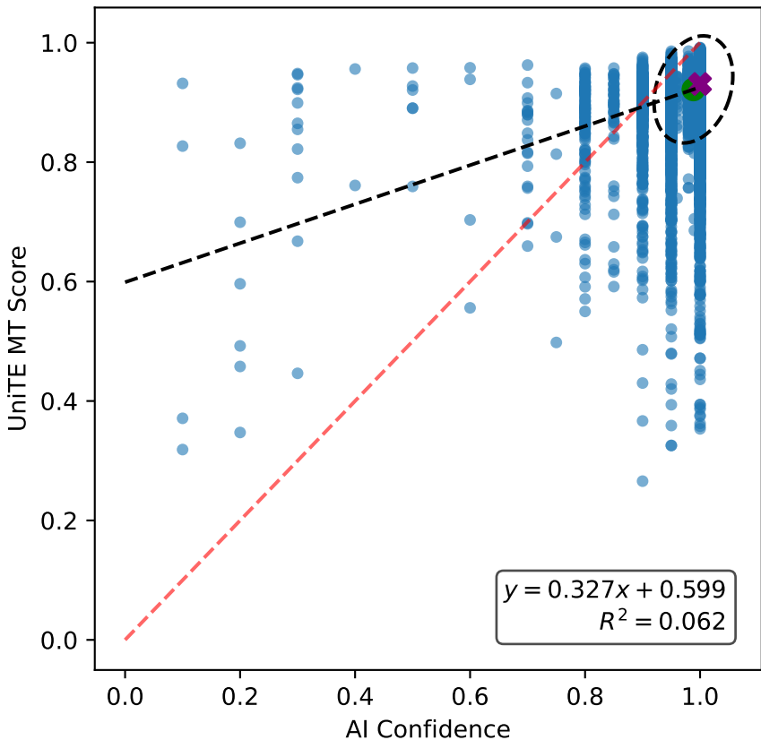
Calibration of Qwen3-14B thinking on Chinese with iterative prompt
