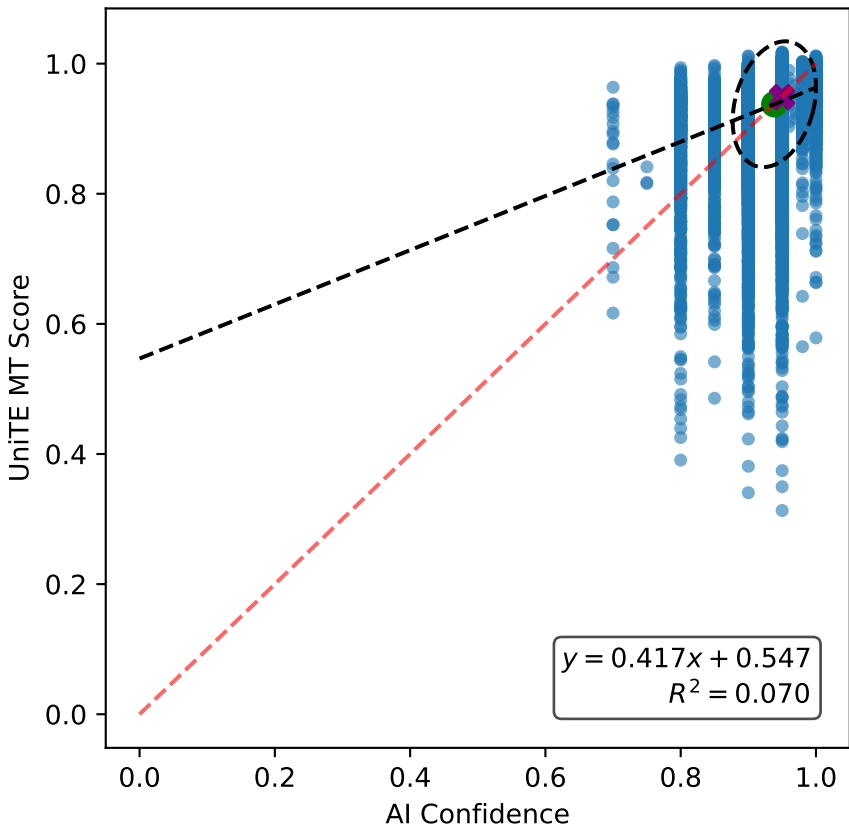
Calibration of Qwen3-14B thinking on Japanese with monolithic prompt
