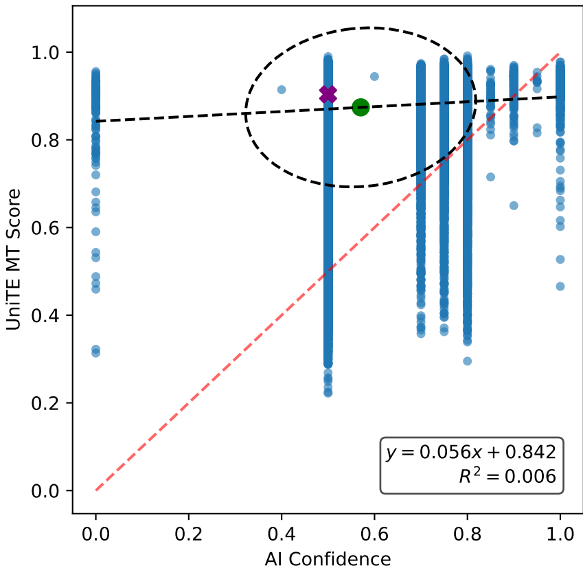
Calibration of Qwen3-1.7B basic on French with iterative prompt
