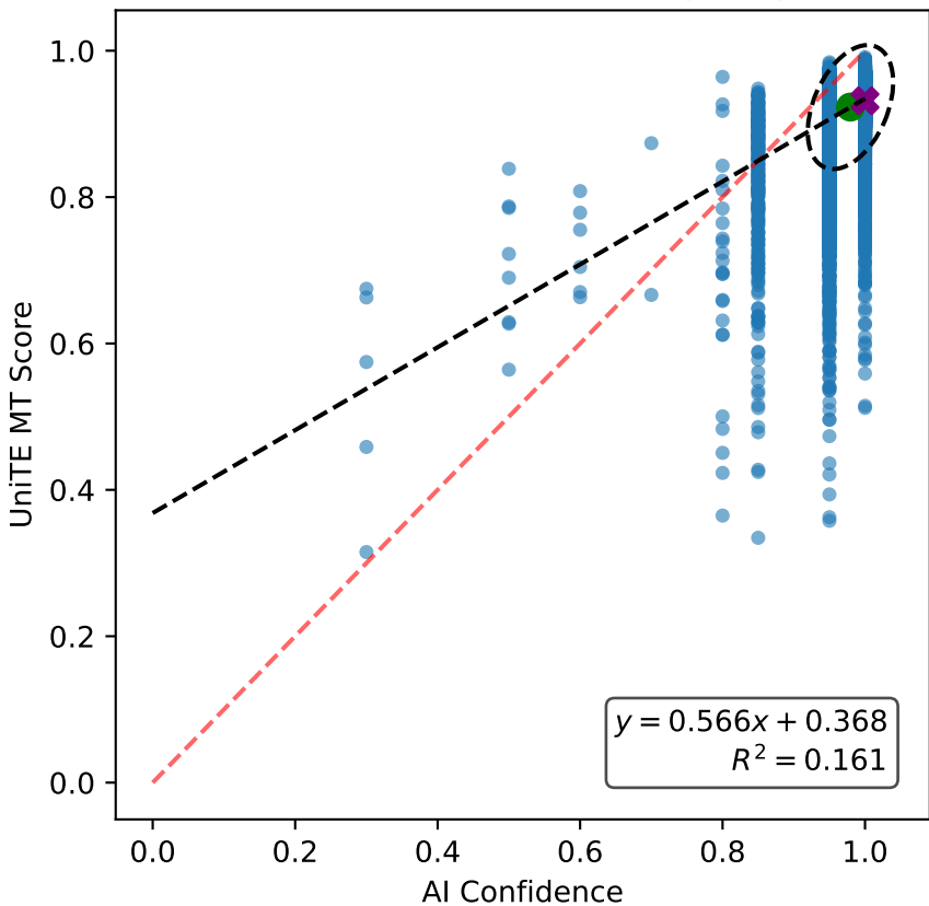
Calibration of Qwen3-14B basic on Chinese with iterative prompt
