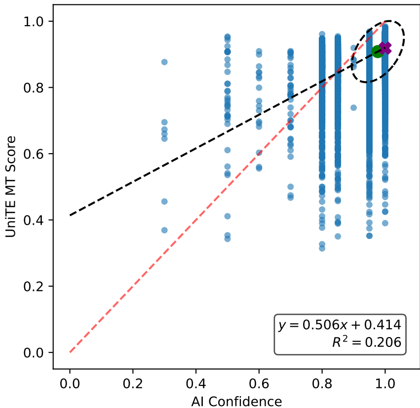
Calibration of Qwen3-14B basic on German with iterative prompt
