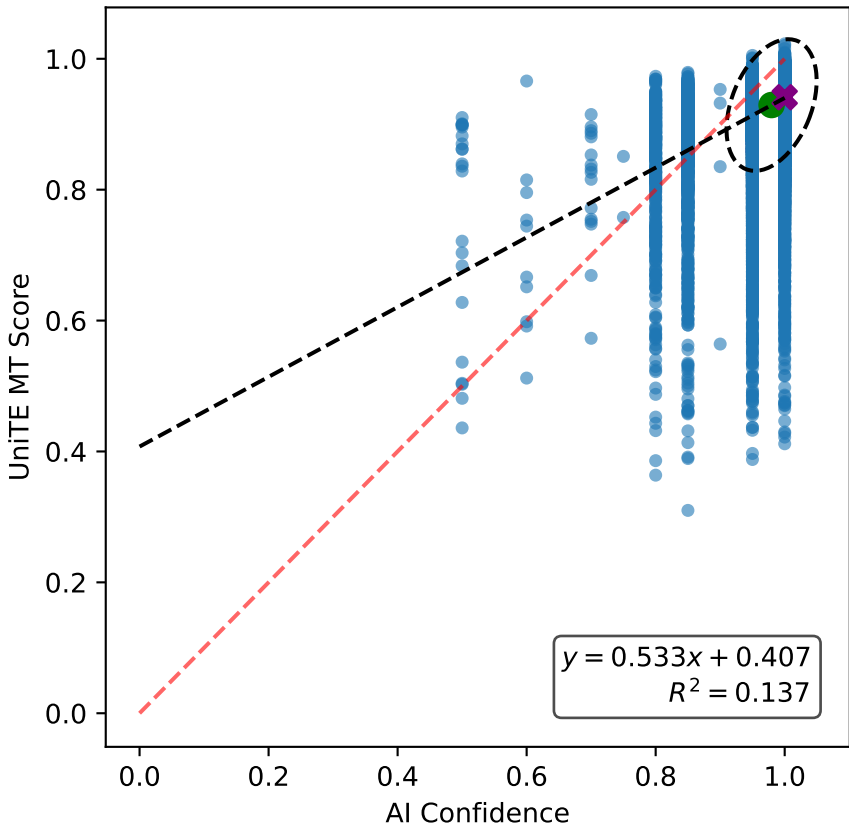
Calibration of Qwen3-14B basic on Italian with iterative prompt
