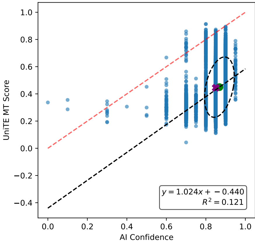
Calibration of Qwen3-14B basic on Berber with monolithic prompt
