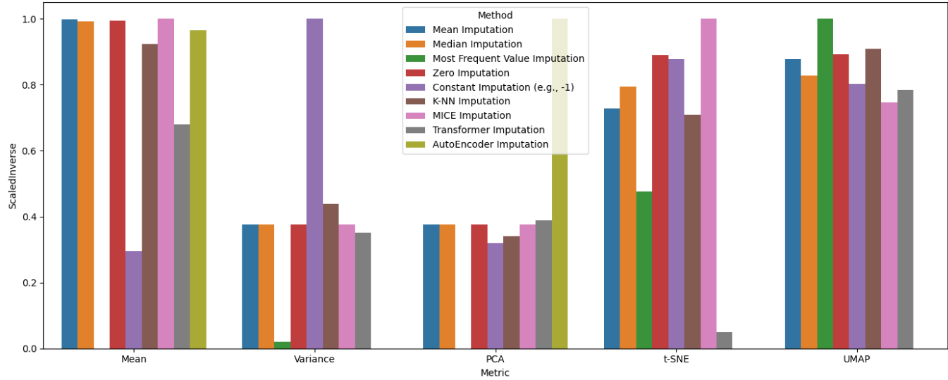
Scaled Inverse Scores Across Evaluation Metrics (Higher is Better)
