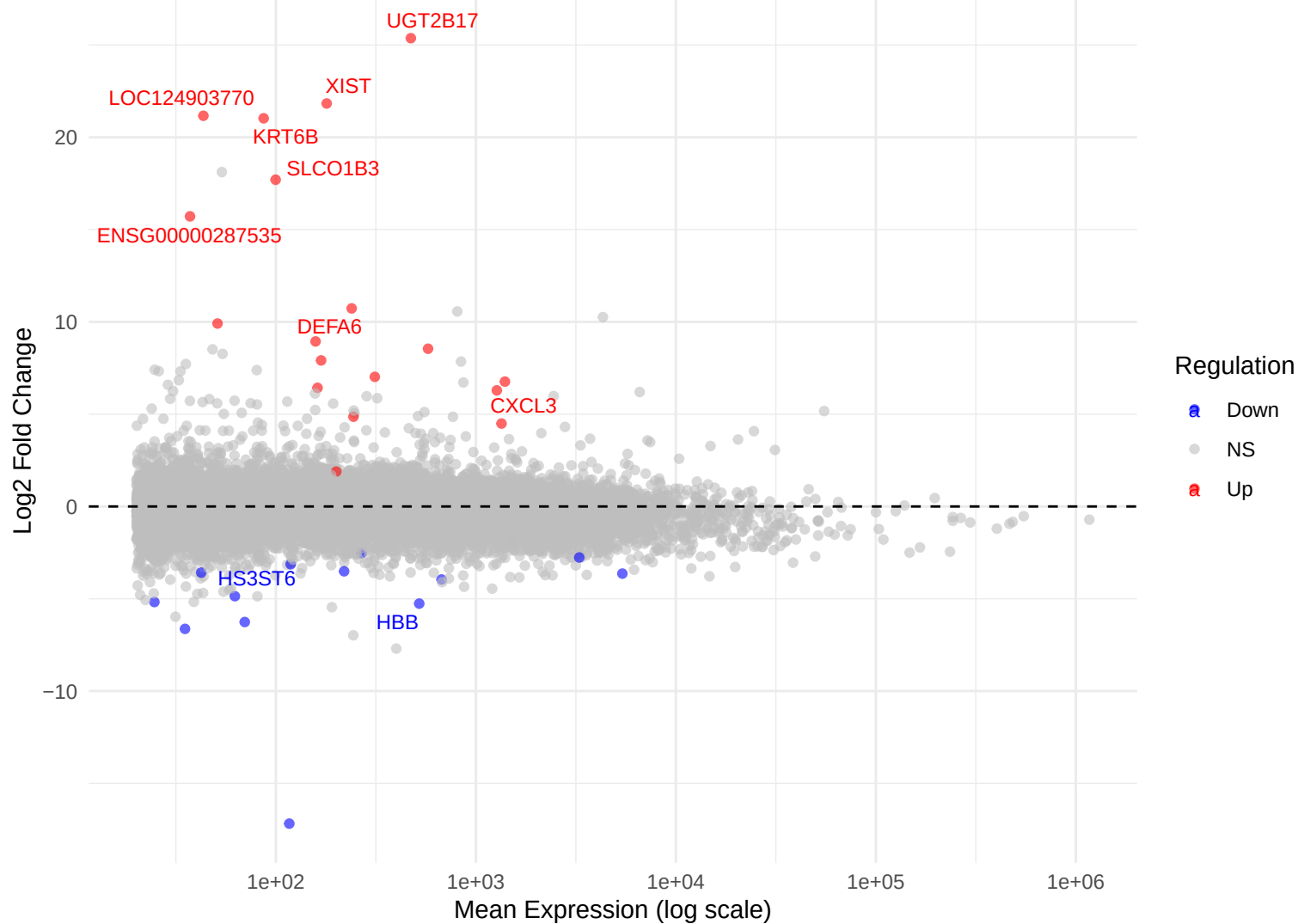
MA Plot: Early Stage Tumor vs Advanced Tumor
