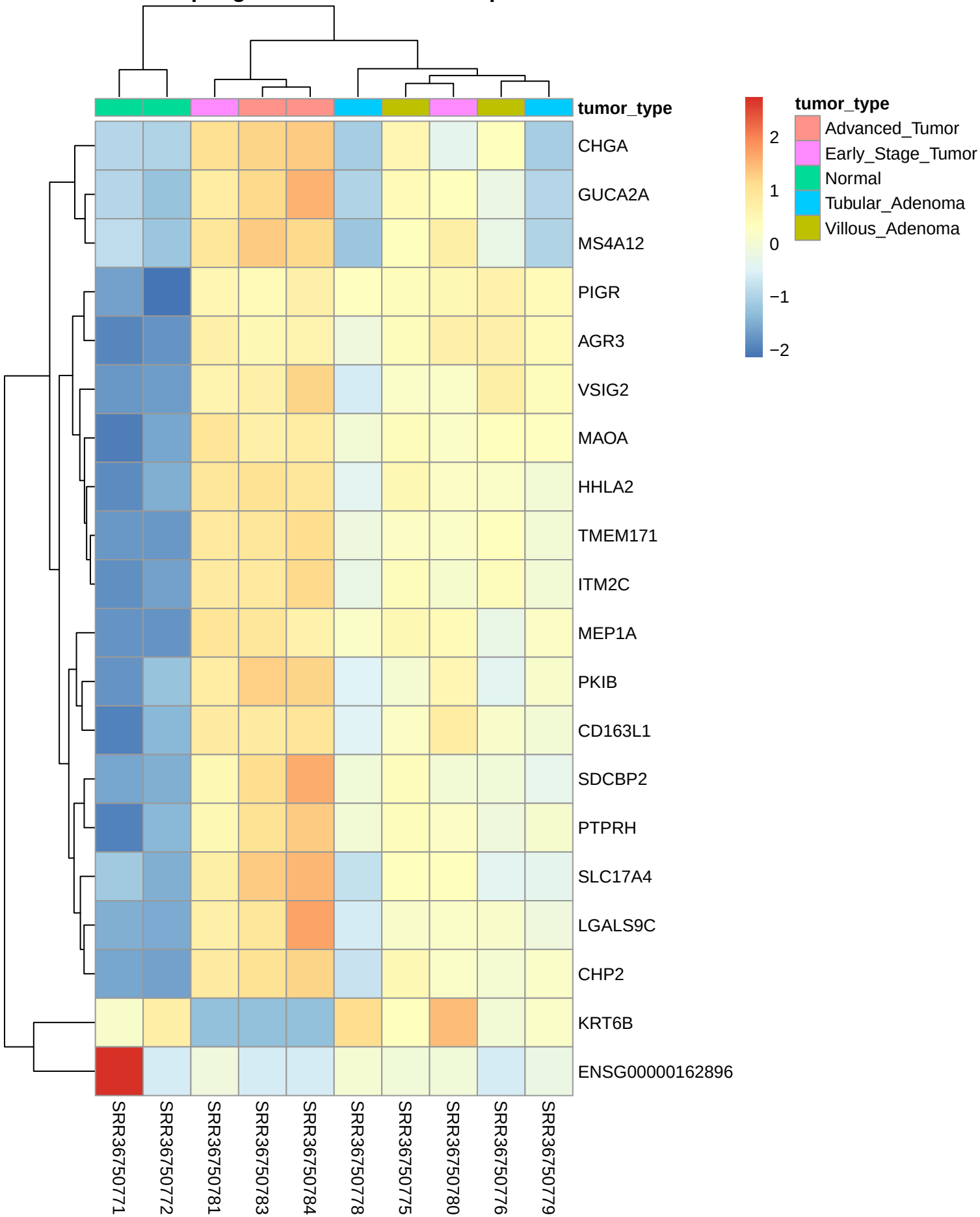
Top Significant Genes Heatmap
