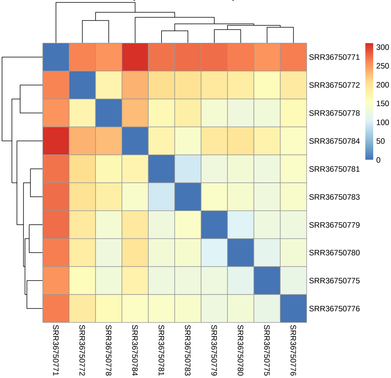
Sample Distance Heatmap
