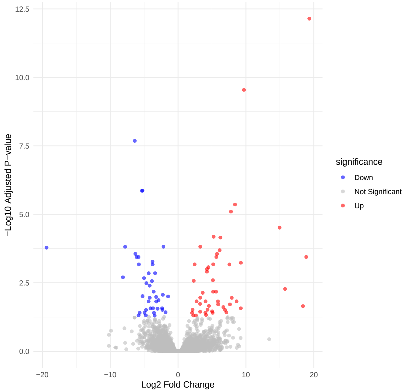
Volcano Plot
