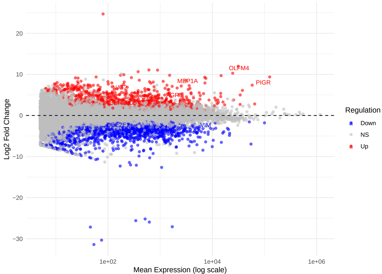
MA Plot: Tubular Adenoma vs Early Stage Tumor
