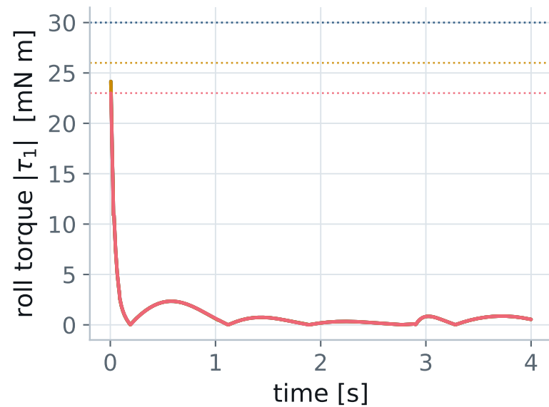
(b) the applied torque respects them
