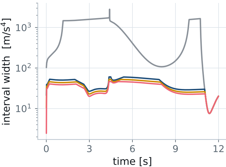
(a) the bounds narrow the interval
