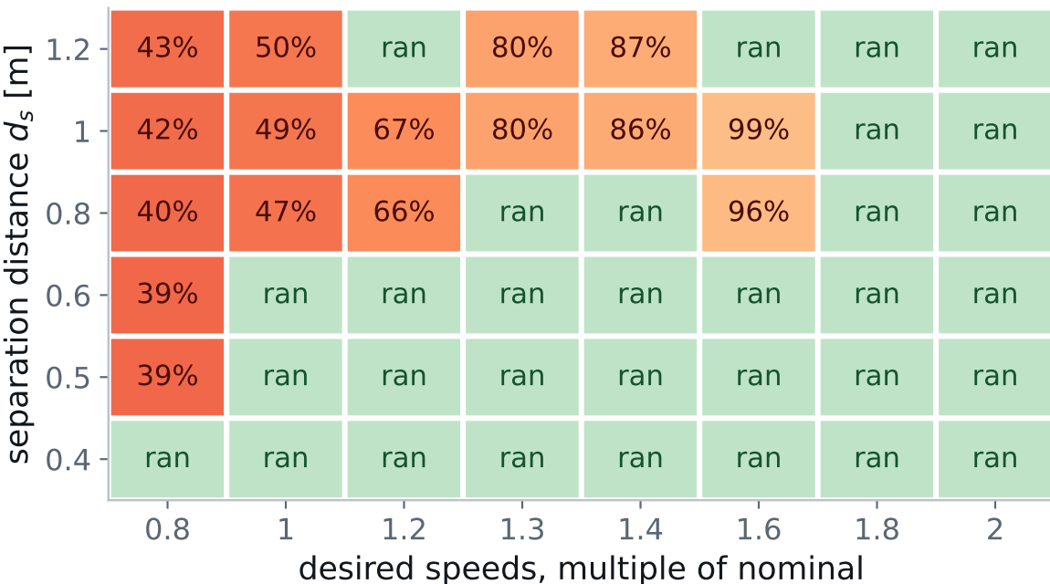
(a) two quadrotors, intersecting sinusoids
