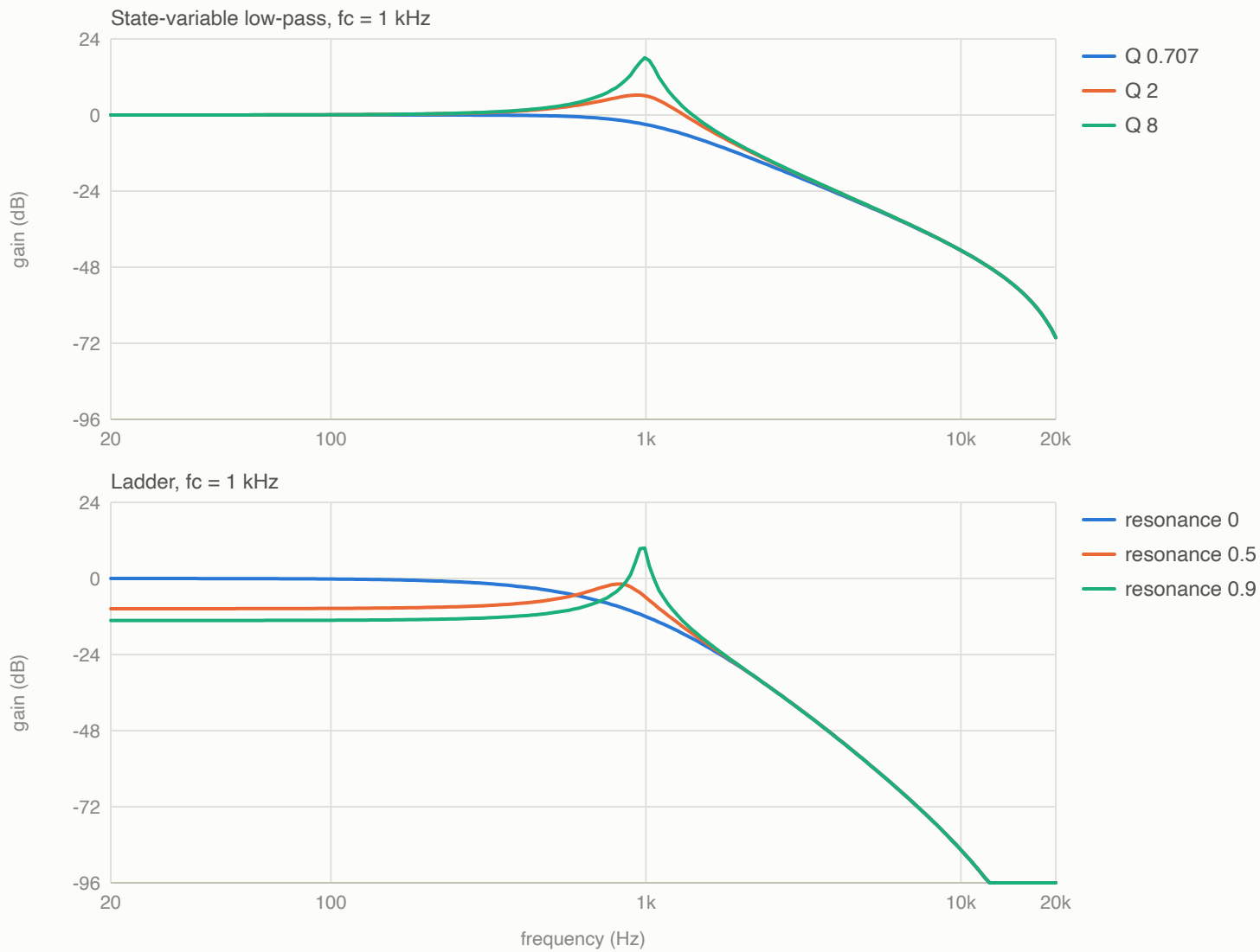
Figure 3. Magnitude responses of the two TPT filters
