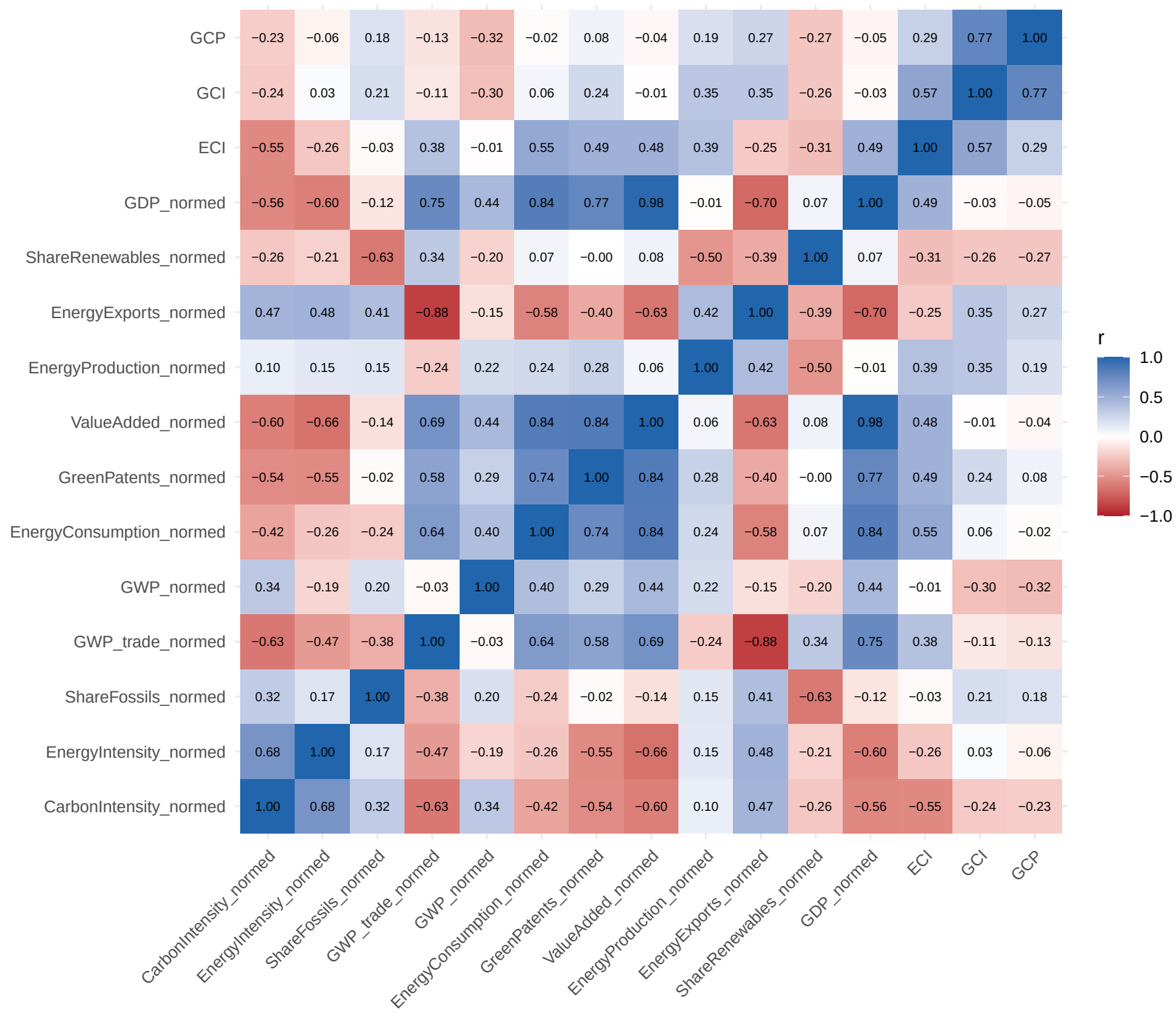
Indicator correlations
