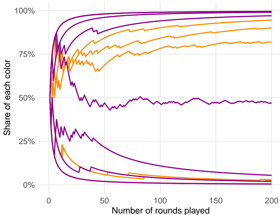
Polya Urn (pr. replacement II): Typical runs
