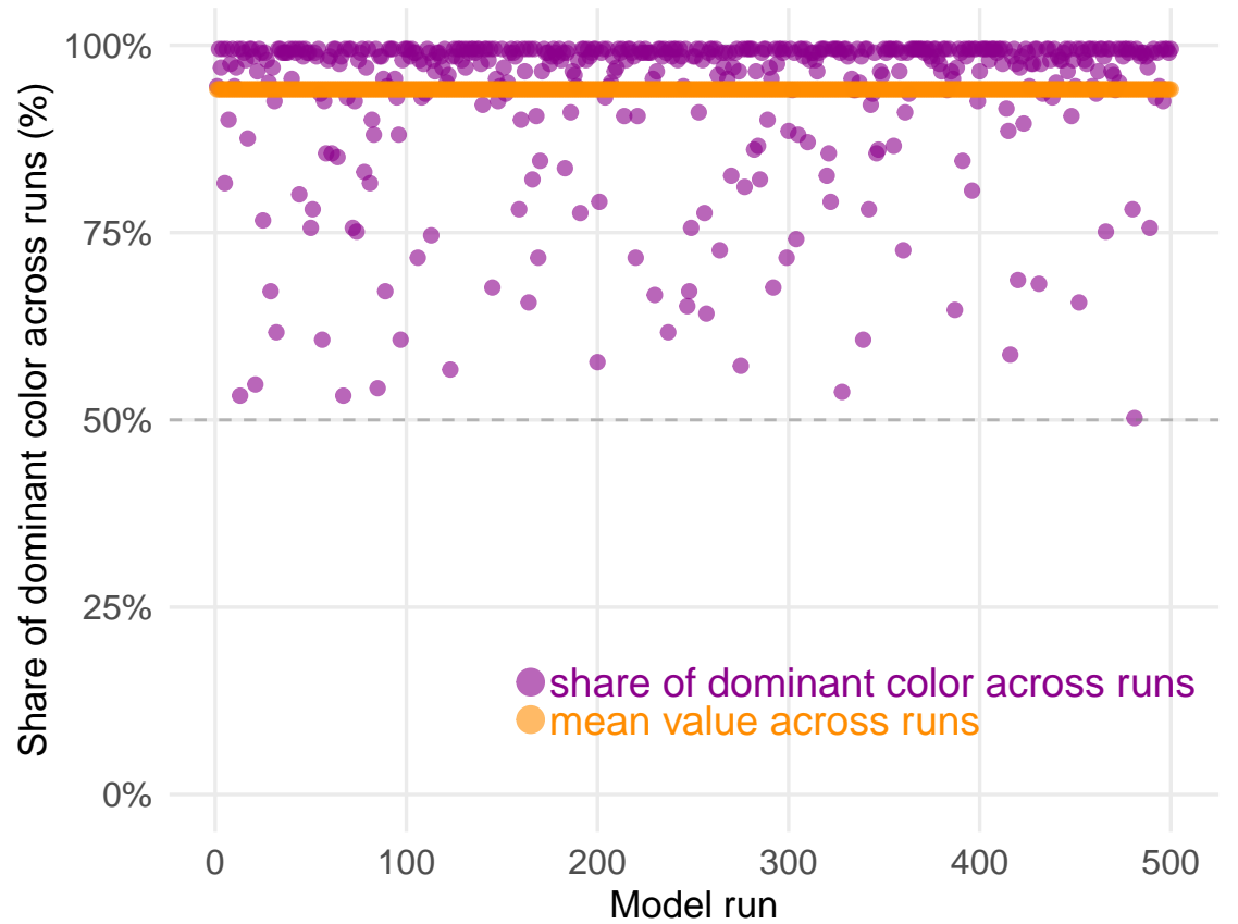
Polya Urn (pr. replacement II): Distribution of outcomes
