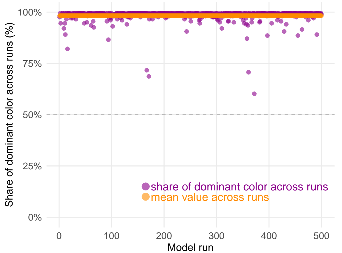
Polya Urn (prob. replacement): Distribution of outcomes
