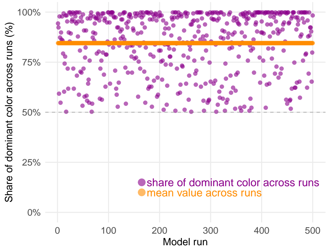
Polya Urn (higher growth): Distribution of outcomes
