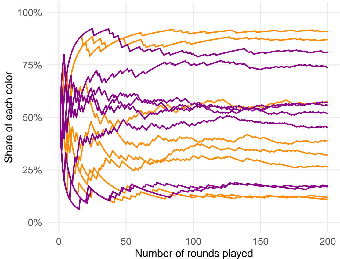
Standard Polya Urn: Typical runs
