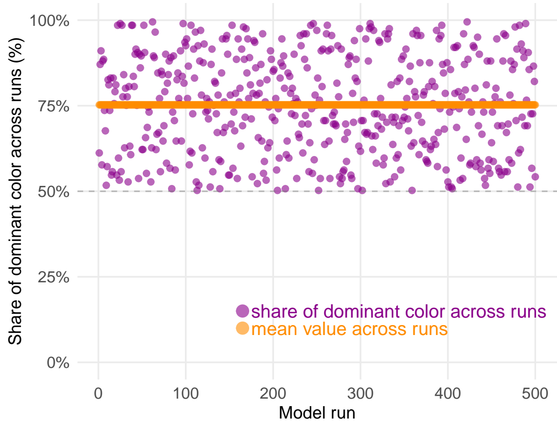
Standard Polya Urn: Distribution of outcomes
