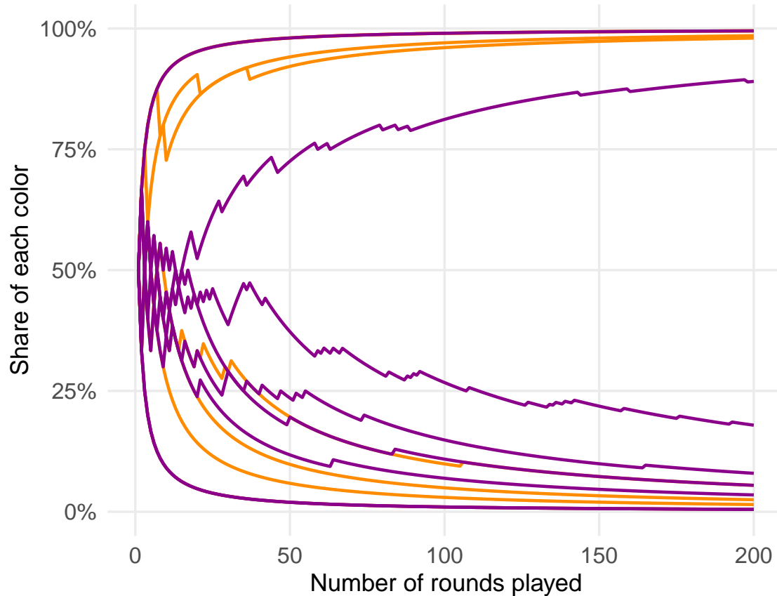
Polya Urn (prob. replacement): Typical runs
