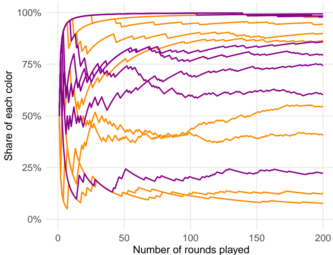
Polya Urn (higher growth): Typical runs
