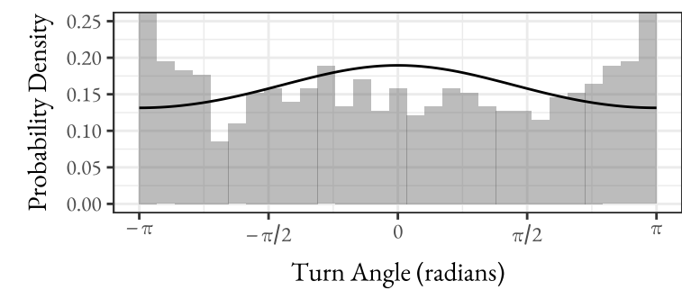
Movement kernel
