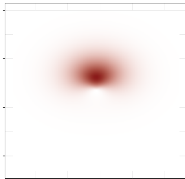
Movement kernel
