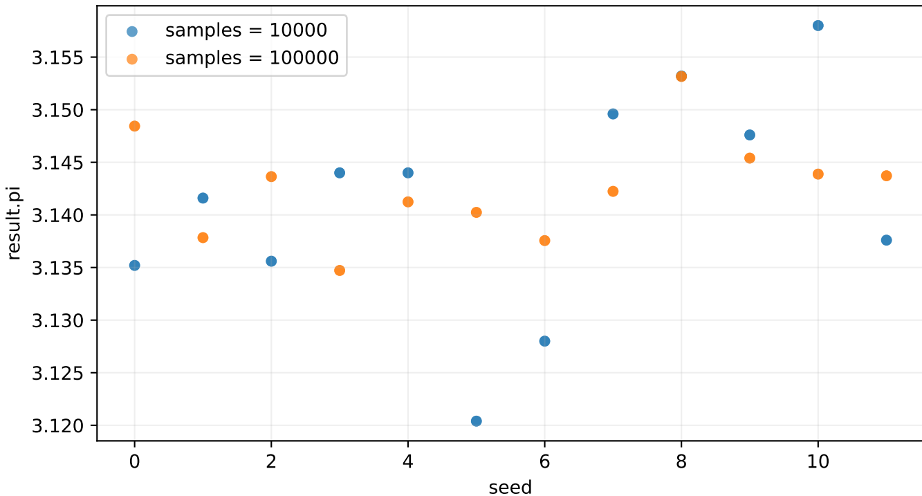
Monte Carlo reproducibility study
