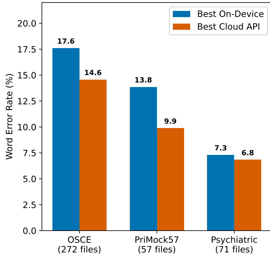
WER (lower is better)
