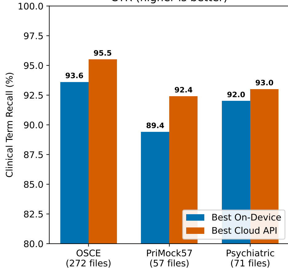
CTR (higher is better)
