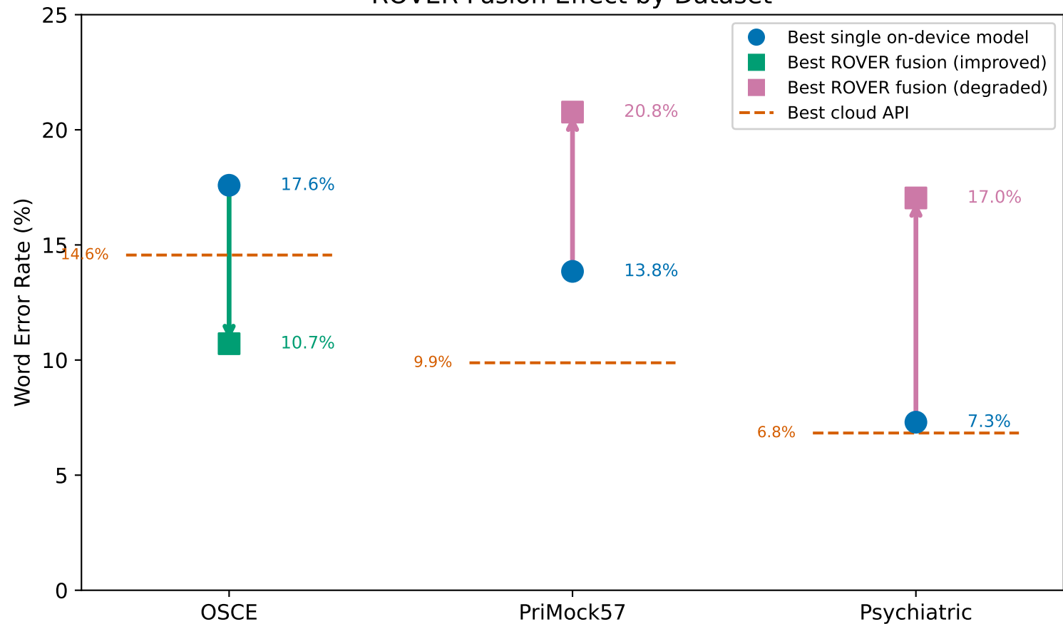
ROVER Fusion Effect by Dataset
