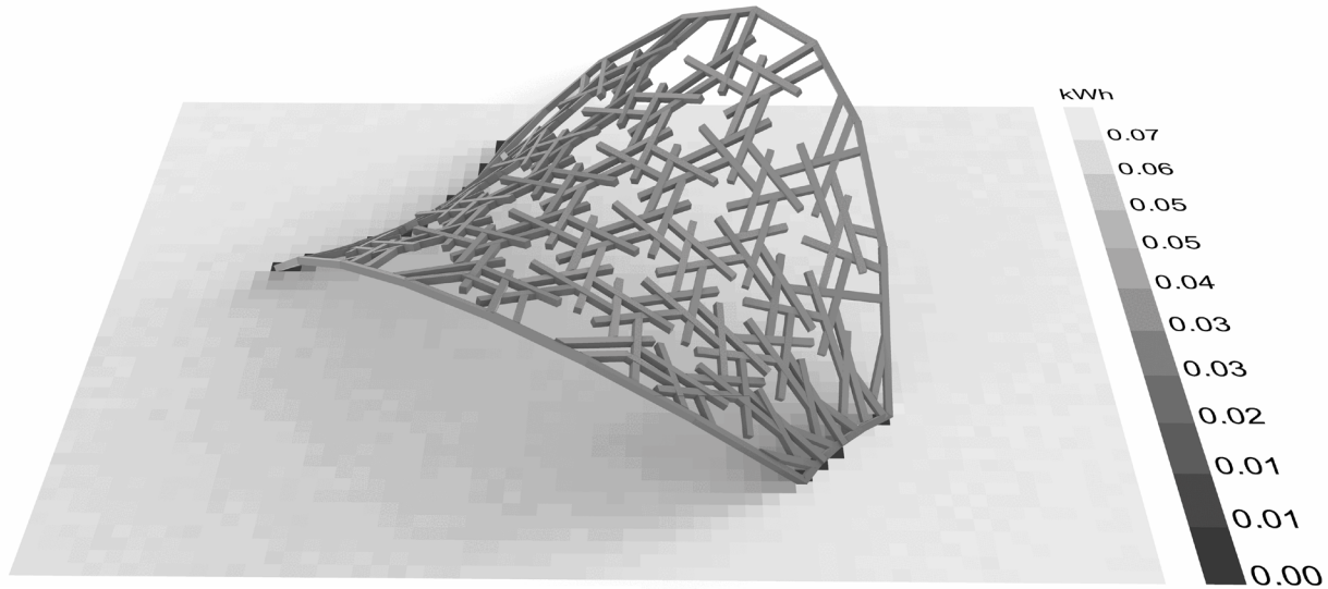
Cumulative Radiation Zurich - 21 June
