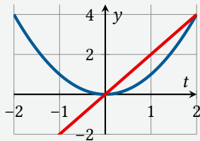
Polynom
