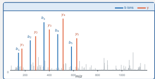
Labeled data
