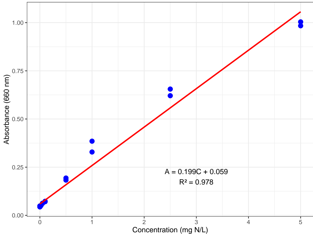
NH 4 + Calibration Curve (Berthelot Reaction)
