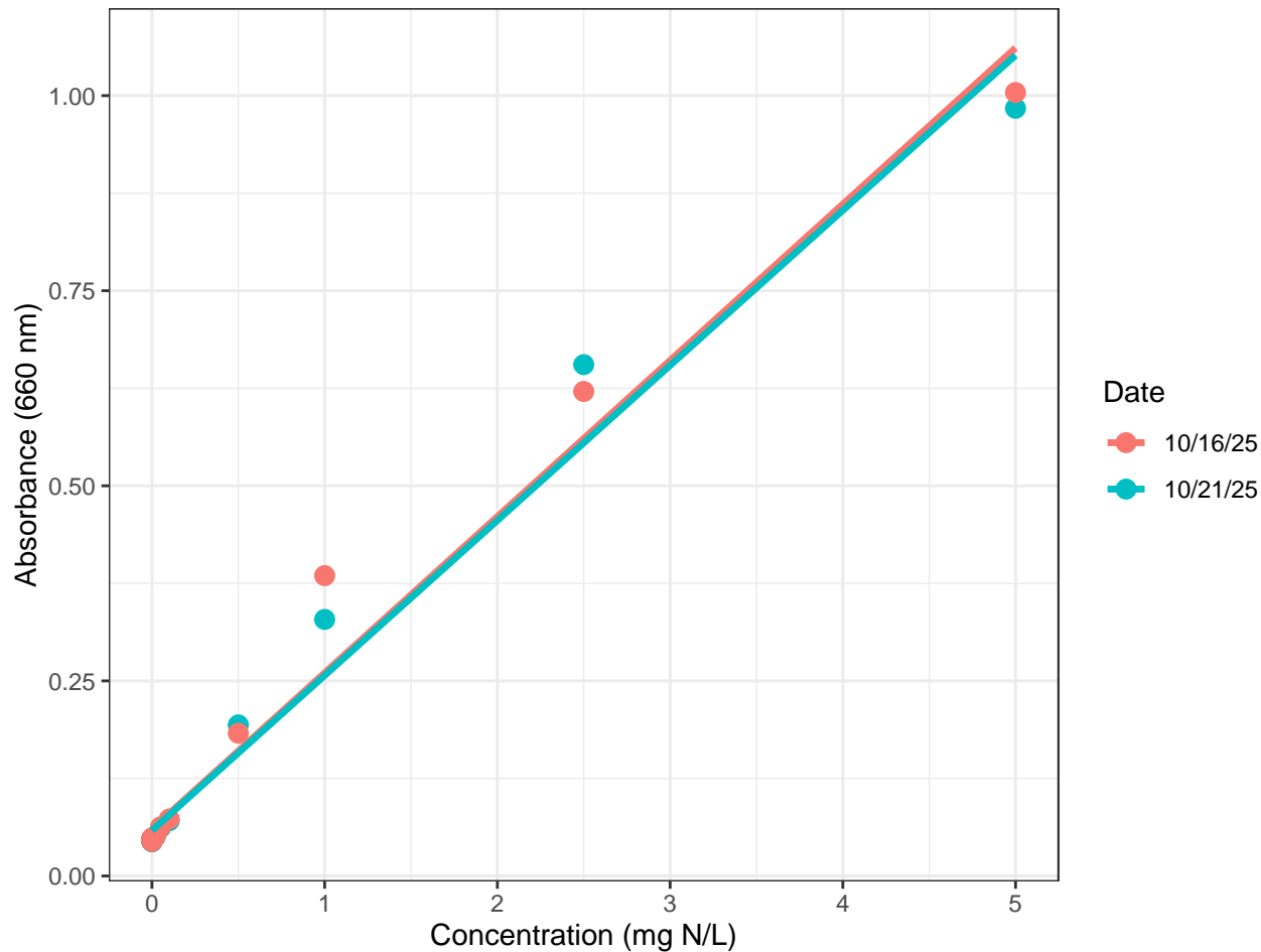
NH 4 + Calibration Curves by Date (Berthelot Reaction)
