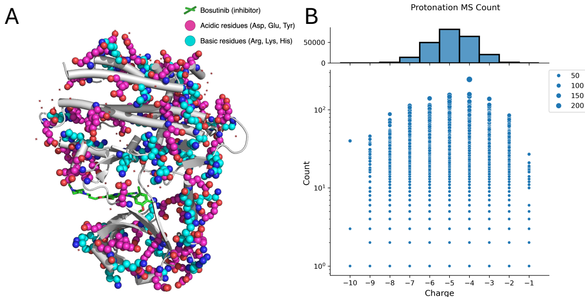
Figure 2: MCCE Microstate Distribution of bosutinib bound to the ABL tyrosine kinase domain. (A) Structure of the ABL tyrosine kinase domain bound to the inhibitor Bosutinib (PDB: 3UE4). The ionizable residues shown as spheres (acids: magenta; bases: cyan) and the inhibitor shown as green sticks. (B) MCCE microstate charge distribution at physiological pH (7.4). The upper histogram shows the total microstate count at each net charge; the lower panel displays sets of unique microstates, with point size proportional to their sampling count in the Monte Carlo ensemble.
