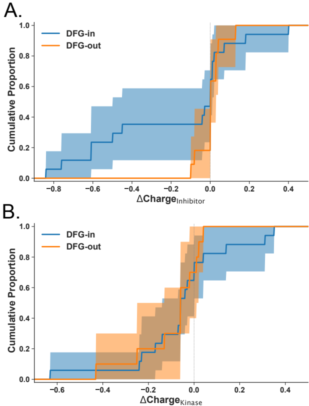
Figure 5: Net-charge changes of inhibitor or kinase do not display strong conformational dependence upon binding. (A) Empirical CDF (ECDF) curves of net-charge changes of all inhibitors split by whether the kinase-state bound is labeled as DFG-in (blue) or DFG-out (orange). Charge changes in both positive and negative directions are shown, alongside no net-charge change (vertical dashed line). 95% confidence intervals (shaded region) are plotted alongside the ECDF.(solid line). (B) Empirical CDF (ECDF) curves of net-charge changes of all kinases split by whether the kinase-inhibitor bound complex has been labeled as DFG-in (blue) or DFG-out (orange). Charge changes in both positive and negative directions are shown, alongside no net-charge change (vertical dashed line). 95% confidence intervals (shaded region) are plotted alongside the ECDF.(solid line).
