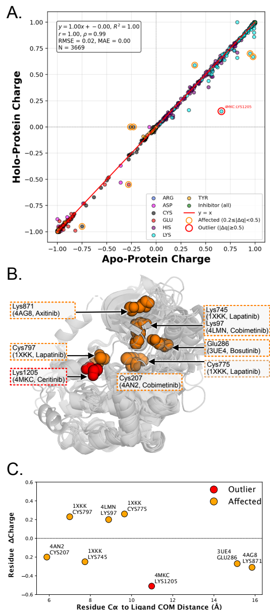
Figure 4: Effect of inhibitor binding on residue charge states across kinase-inhibitor complexes. (A) Calculated average charge of each titratable residue in the inhibitor-bound holo-protein versus apoprotein MCCE simulations at pH 7.4, aggregated across all kinase-inhibitor pairs ( N = 3669 residues from 37 complexes). Points are colored by residue type and the red line denotes identity with no change between apo- and holo-protein. Residues whose charge shifts upon binding are highlighted in two tiers based on |\Delta q| = |q_{\text{holo}} - q_{\text{apo}}| : outlier residues ( |\Delta q| \geq 0.5 ; red open circles, labeled with PDB:residue) and affected residues ( 0.2 \leq |\Delta q| < 0.5 ; orange open circles). (B) Structural overlay of all residues whose charge shifts upon binding are considered "affected" (orange, 0.2 \leq |\Delta q| < 0.5 ), or "outlier" shifts (red, |\Delta q| \geq 0.5 ). All kinase structures with affected or strong residue changes are overlaid (gray cartoon), showing the charge-shifted residue from A in the respective color. For each charge-shifted residue, the residue identity, position in sequence, PDB ID and corresponding inhibitor are provided (box and arrow). (C) Distance dependence of affected (orange) and outlier (red) residues on the charge change of residue upon binding. Distance is measured inhibitor center of mass ("Ligand COM"), to the residue C \alpha atom. The corresponding PDB and residue index for each point are labeled.
