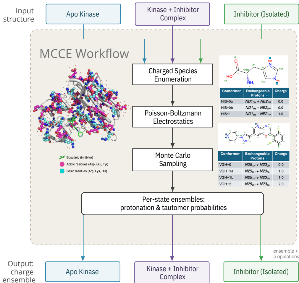
Figure 1: MCCE Workflow. Row 1: MCCE4 calculations are performed independently on three systems: (1) the apo kinase (inhibitor removed), (2) the holo kinase (inhibitor bound), and (3) the inhibitor in solution. Row 2: Conformers are generated to sample protonation states (amino acids and inhibitor), tautomers (His and inhibitor), and polar proton orientations (amino acids). Left panel: Human Anaplastic Lymphoma Kinase in complex with Crizotinib (green sticks) (PDB ID: 2XP2), with spheres highlighting ionizable residues whose charge states can change (acids: magenta; bases: cyan). Right panel: The conformer tables illustrate the protonation and tautomer states sampled for His and for the inhibitor Crizotinib (see SI Fig. 1 for other inhibitors). Each His has one charged (+1) and two neutral tautomers. Crizotinib conformers span net charges from 0, +1 or +2; subscript notation (0H, 1H, 2H) indicates the number of protons on each nitrogen, with labile nitrogens labels highlighted in red in the chemical structures. Row 3: Poisson-Boltzmann electrostatics calculations generate energy lookup tables comprising self-energies (solvation, torsion, and interactions with backbone dipoles) and pairwise conformer-conformer interactions. Row 4: Monte Carlo sampling is performed over microstates, where each microstate represents a unique combination of one conformer per residue and/or ligand. Row 5: Boltzmann-weighted conformer probabilities are obtained, yielding protonation and tautomer populations for each system. Row 6: Comparison of the outputs across the three input structures reveals inhibitor-induced changes in residue charge states.
