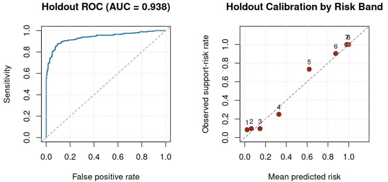
Figure 4: ROC and calibration diagnostics
