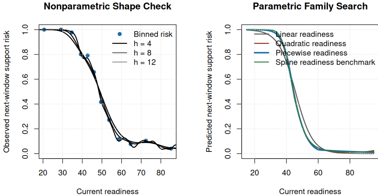
Figure 1: Nonparametric and parametric shape discovery
