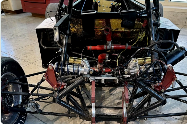
The chassis the radiator had to live in. It was not designed around it.
