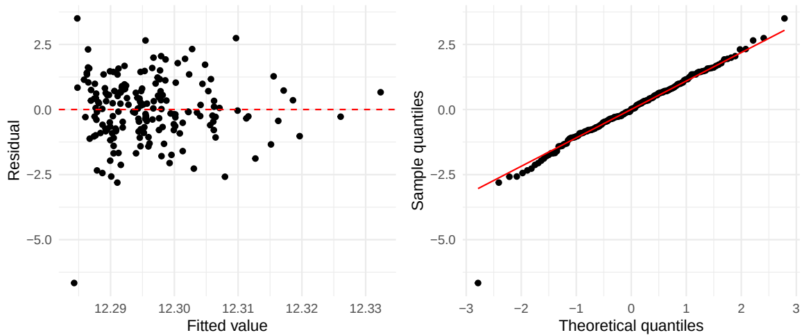
Figure 7: Residuals vs. fitted values and normal QQ plot of residuals for the log-transformed model.
