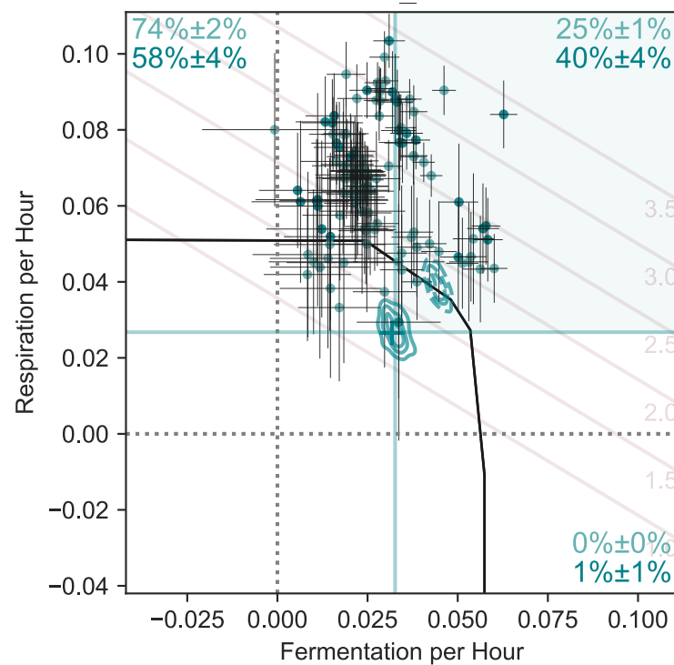
IRA1-missense second-step
