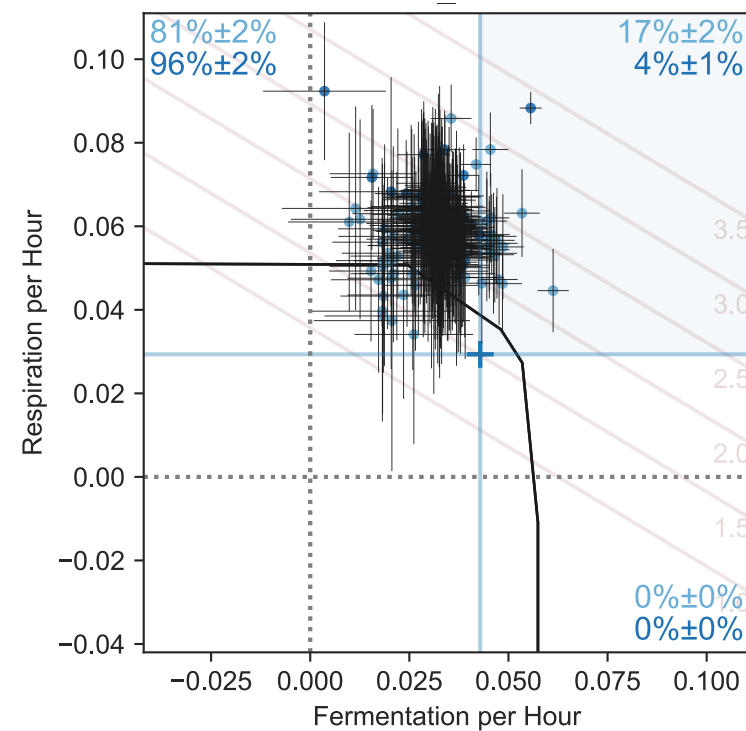
IRA1-nonsense second-step
