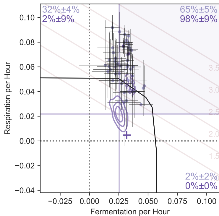
TOR1 second-step
