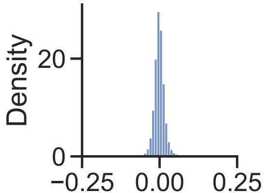
ResNet50
