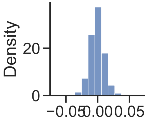
AlexNet
