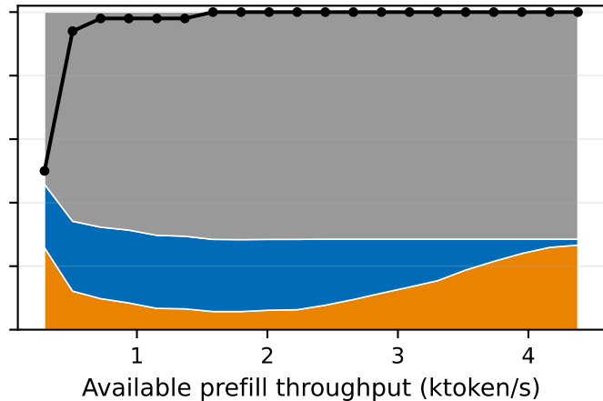
Prefill sweep Bandwidth fixed at 4.87 Gbit/s
