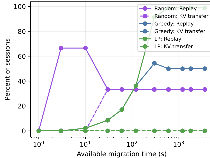
Actions chosen
