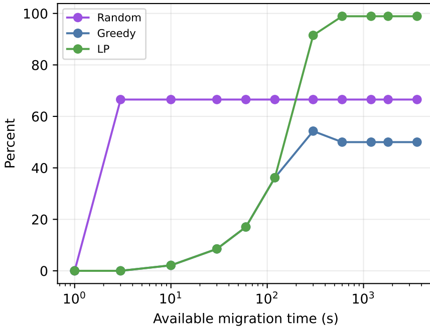
Sessions selected
