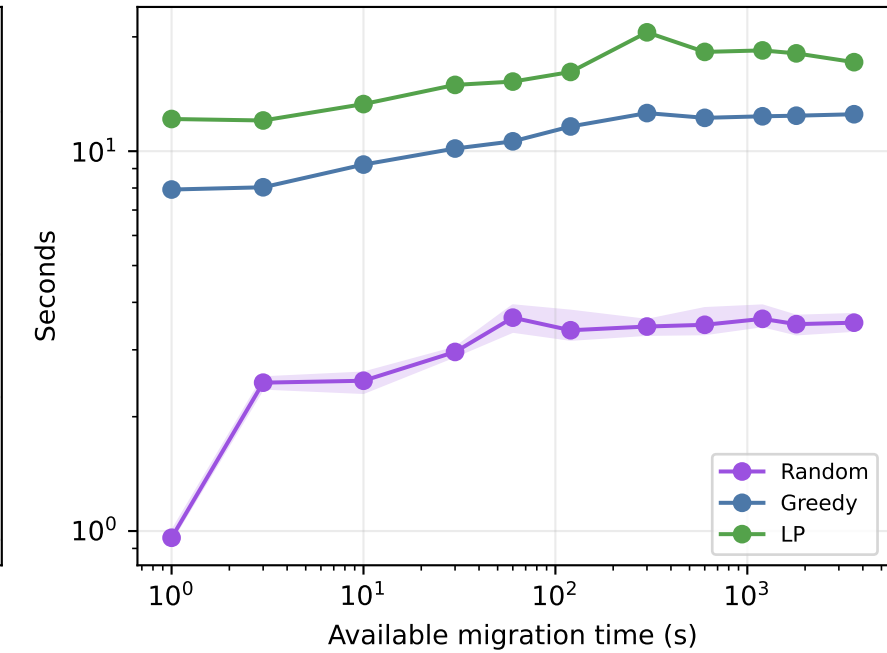
Planning time
