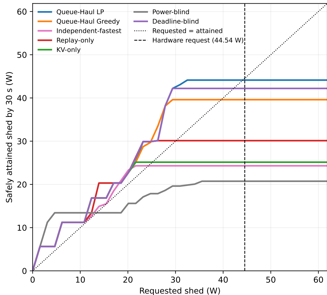
All-bind attainment frontier
