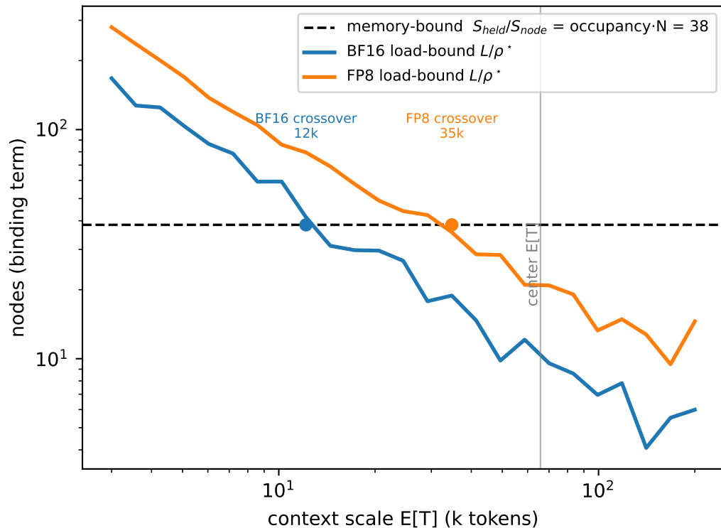
Regime walk: load \rightarrow memory crossover (measured)
