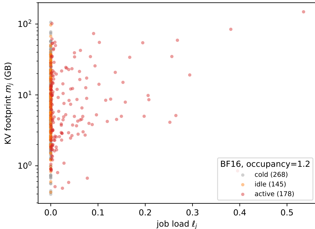
Population in (load, memory): N=591 , E[T]=66,243
