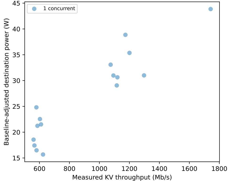
kv transfer
