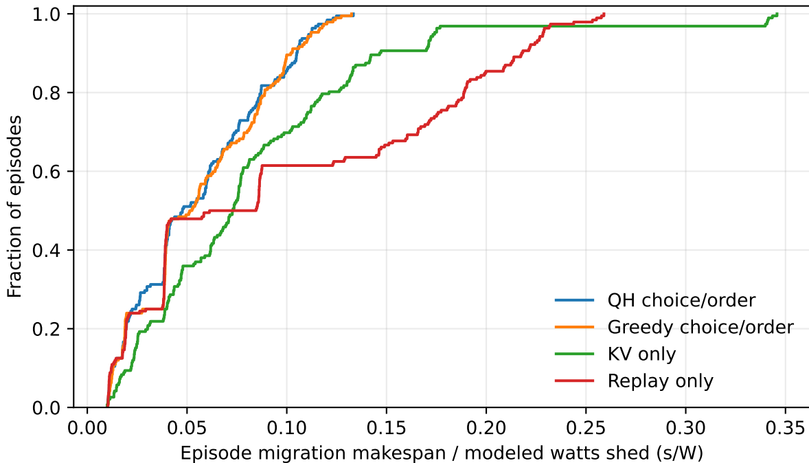
Width-8 hardware migration time per watt (768 episodes)
