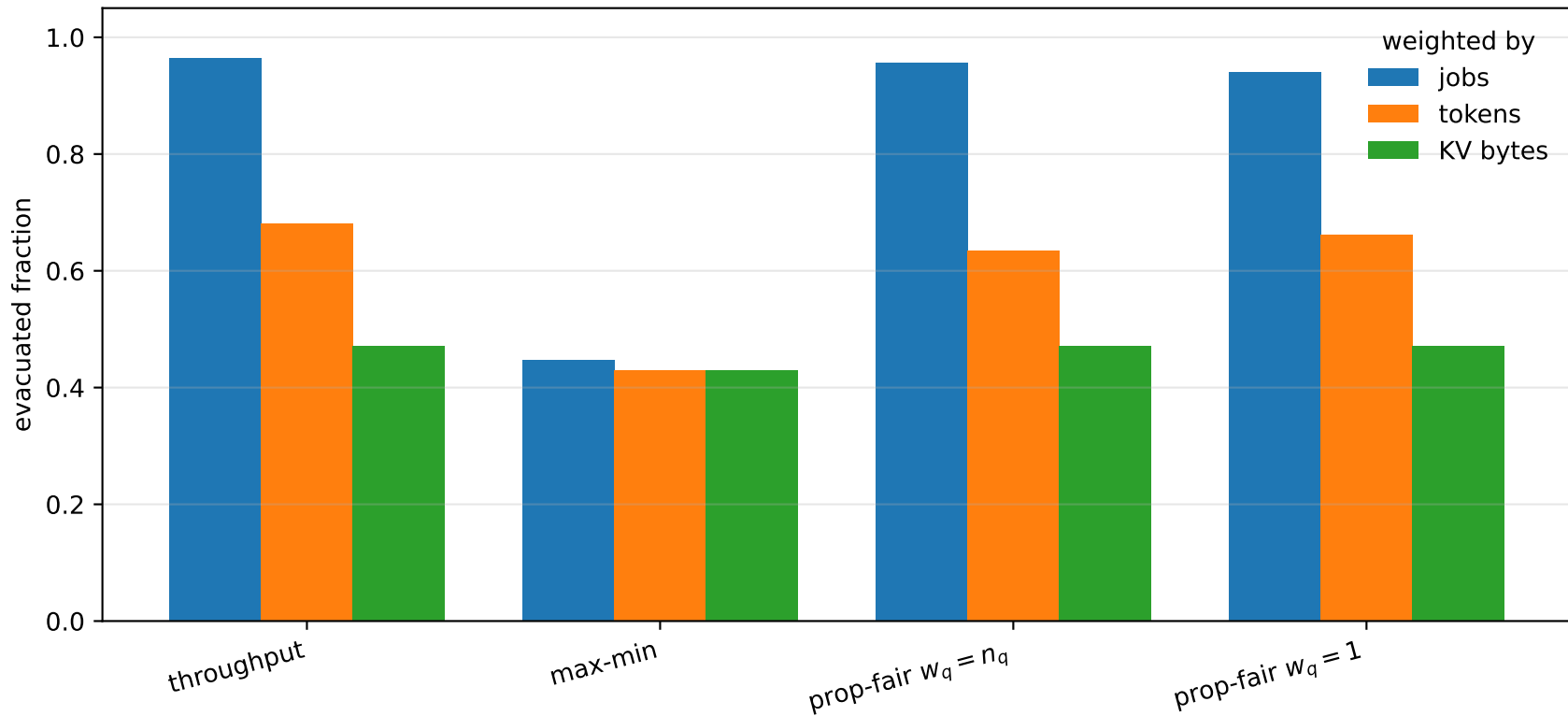
Evacuation weighted by jobs vs tokens vs KV bytes, D = 120.0s
