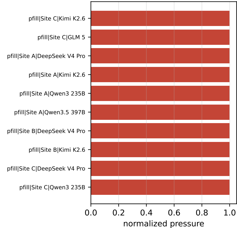
max-min ( \phi^* = 1.000 )
