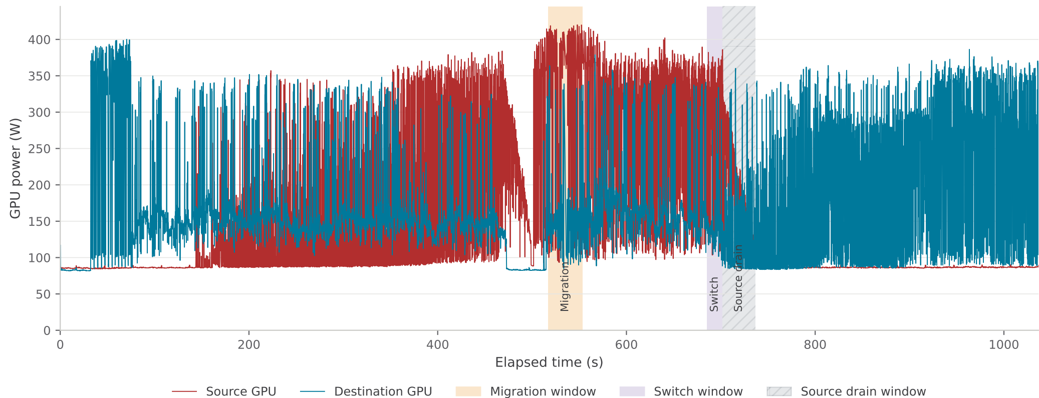
Full-shed migration under live load: source 4 rps, destination 1 rps
