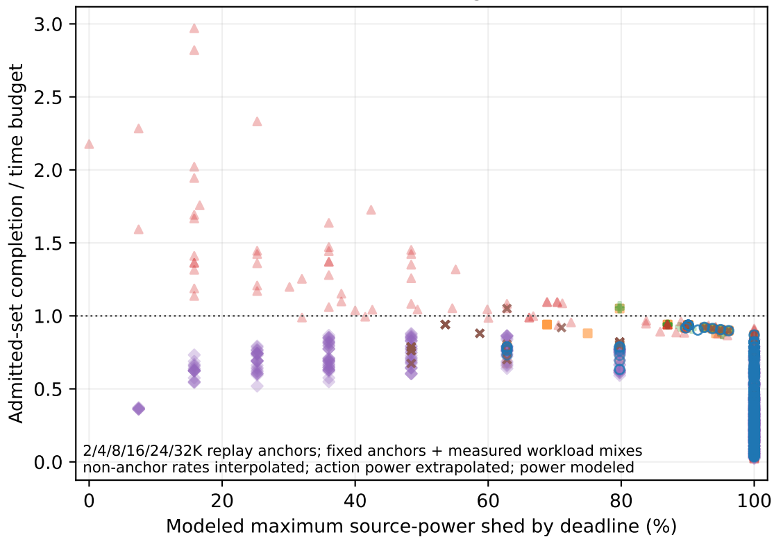
Matched scenario-budget outcomes
