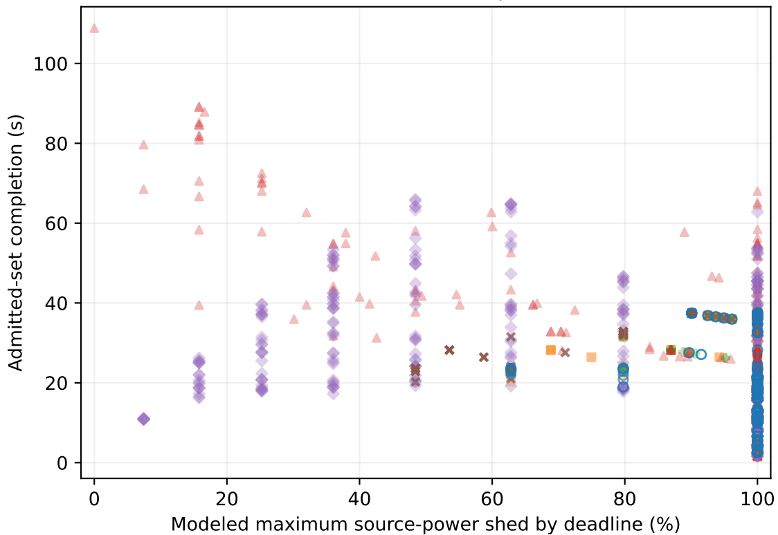
All admitted-set completions
