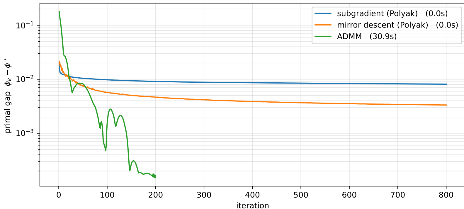
Stage 2 dual decomposition: per-class subproblems at given prices Q = 200 classes, |\mathcal{I}| = 39 pressure indices, \phi^* = 0.0135 (CVXPY ground truth)
