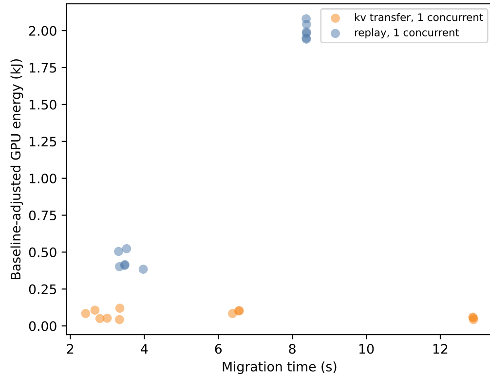
Time and measured GPU energy
