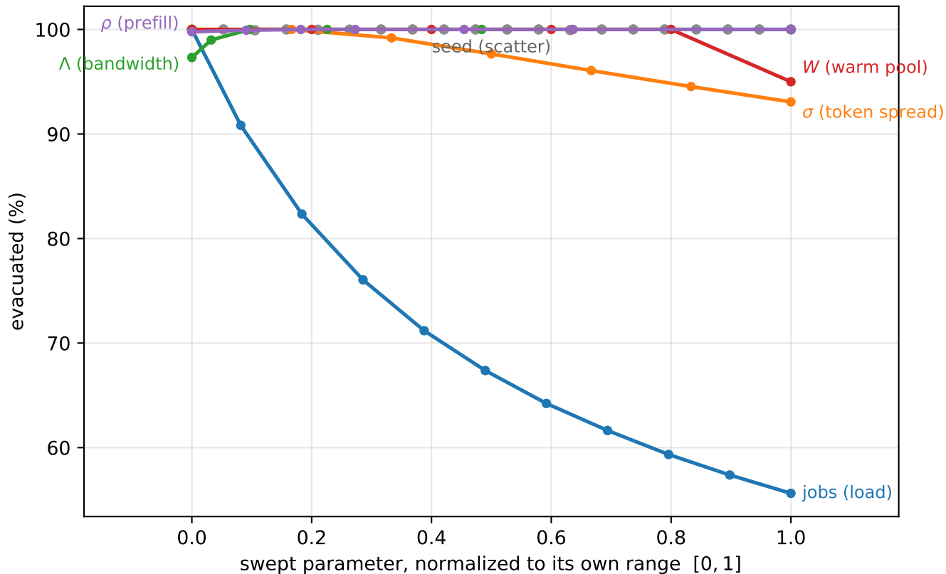
Sensitivity fan: evacuation fraction vs each swept parameter
