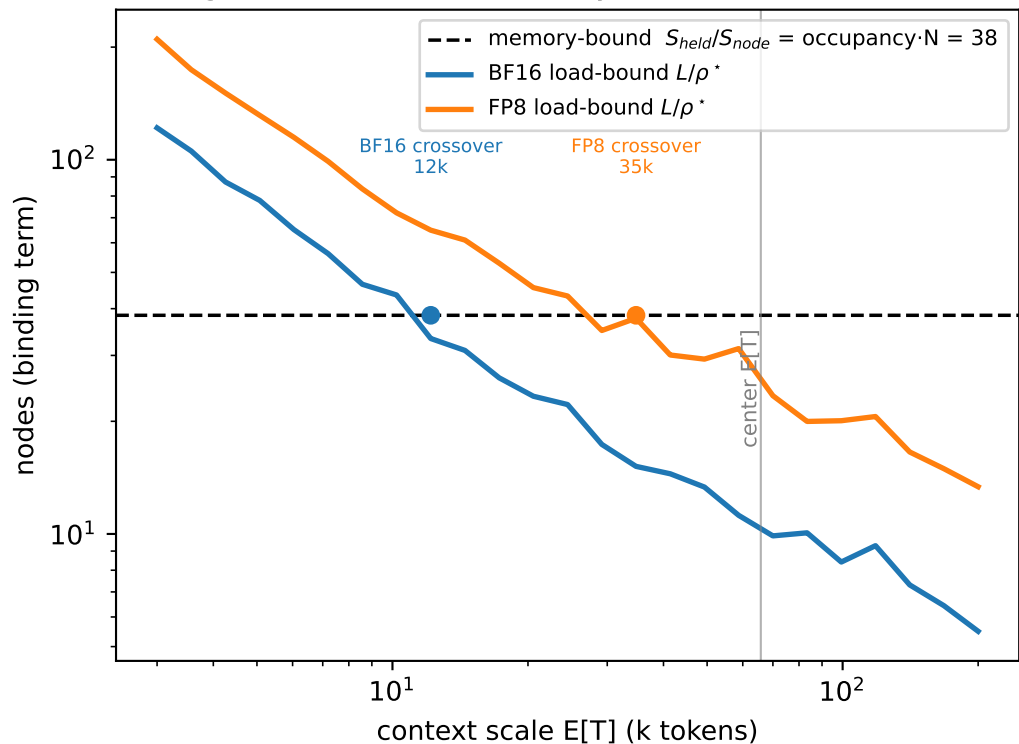
Regime walk: load→memory crossover (measured)
