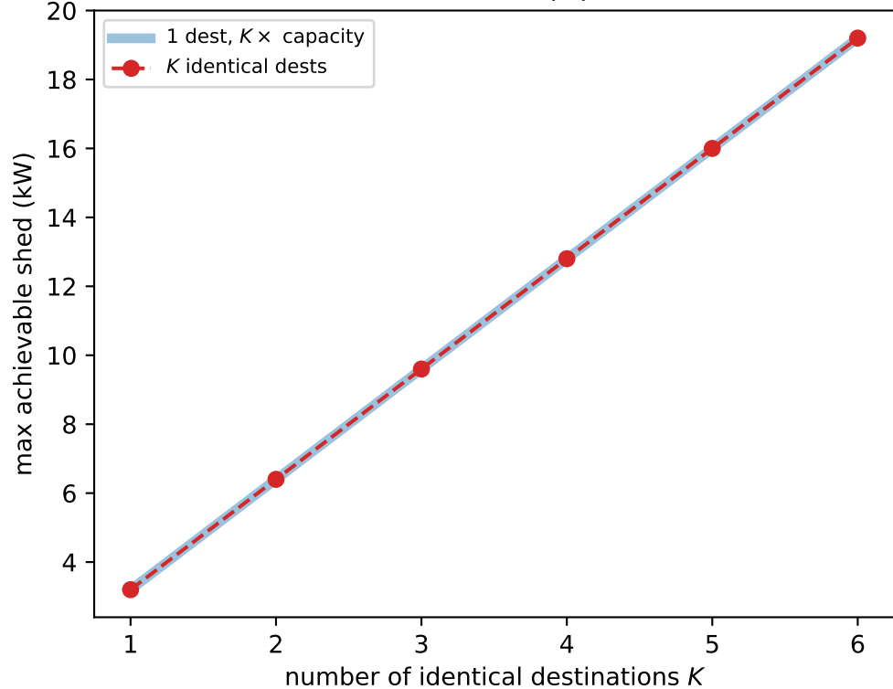
B. split \equiv merged ( \max |\Delta| = 7.1e-15 kW)
