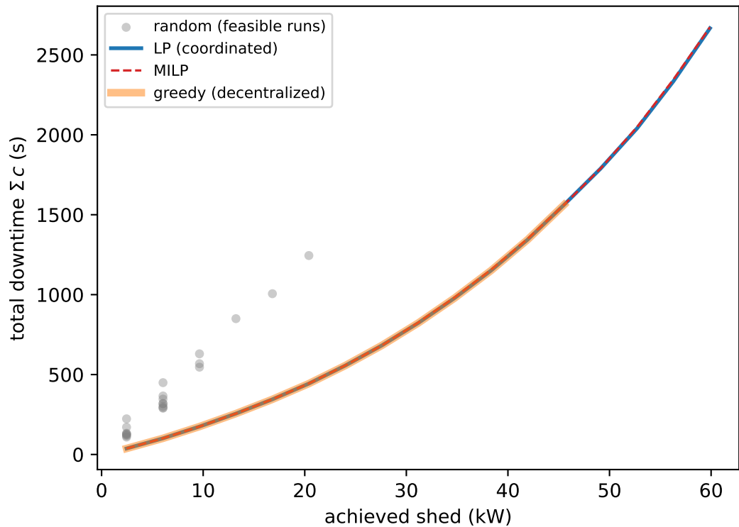
Greedy is local; LP keeps going after the shared link binds
