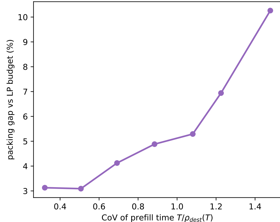
C · gap grows with context heterogeneity ( W=8 )
