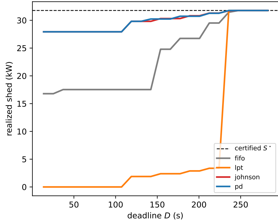
A · grid relief: order-blindness wastes shed
