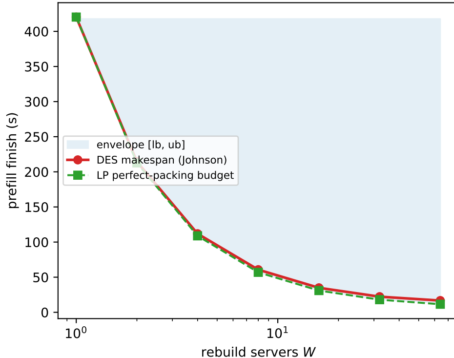
B · P\|C_{max} gap opens as W grows
